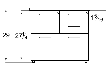
Pedestal Front Profile Multi-File
